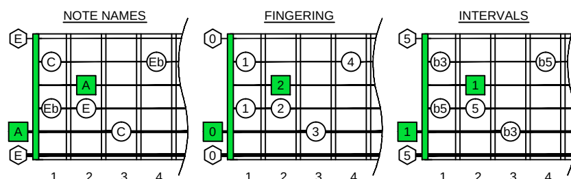
A minor-diminished arpeggio SEMITONOMETER
