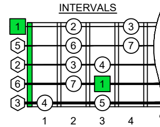
INTERVALS
